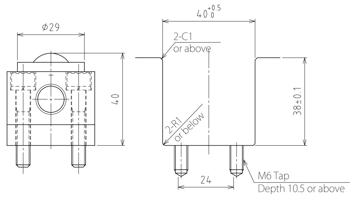
View A Rising (stroke 4mm) Recommended groove dimensions (Scale 1:1)
