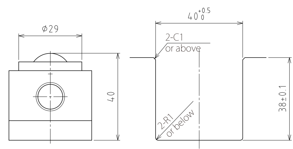
Rising (stroke 4mm) Recommended groove dimensions (Scale 1:1)
