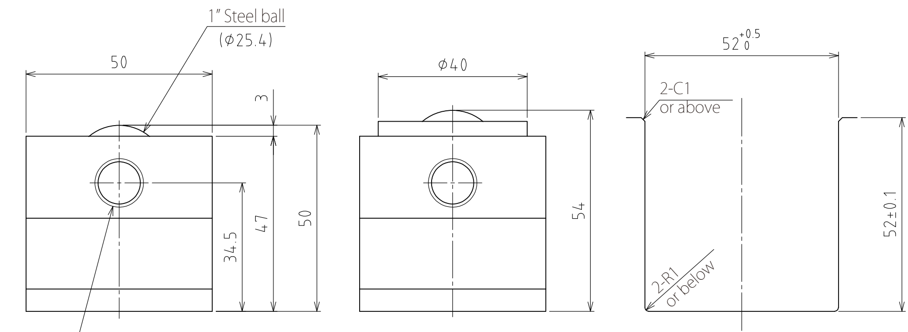
View A Rising (stroke 4mm) Recommended groove dimensions (Scale 1:1)
