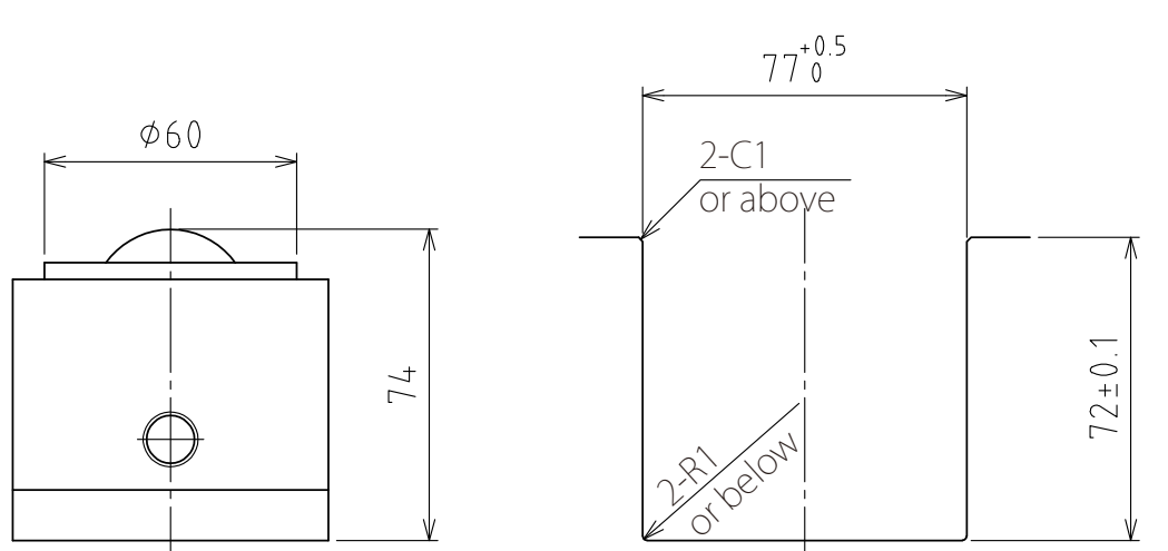
Recommended groove dimensions
