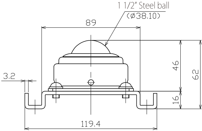
View A (SCALE 1:3)
