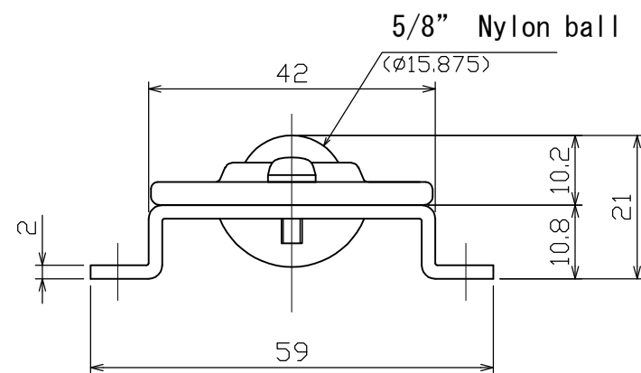
View A (SCALE 1:1)
